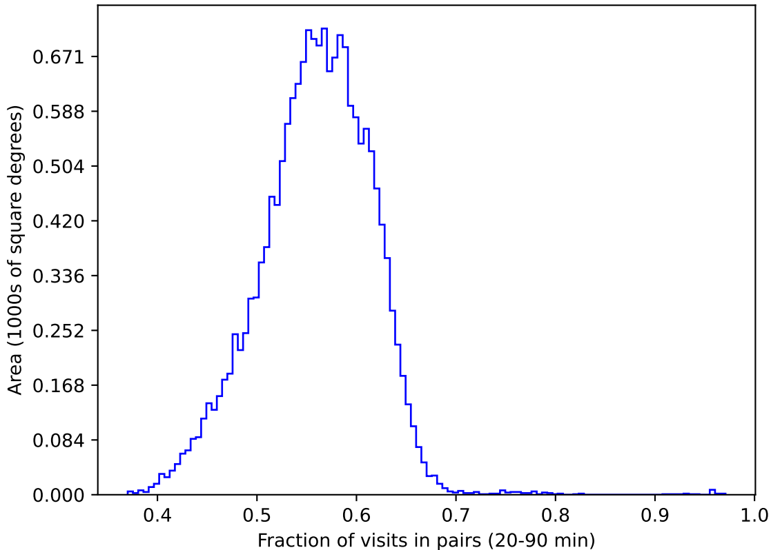
retro_baseline_v2.0_10yrs gri WFD: Fraction of visits in pairs (20-90 min)
