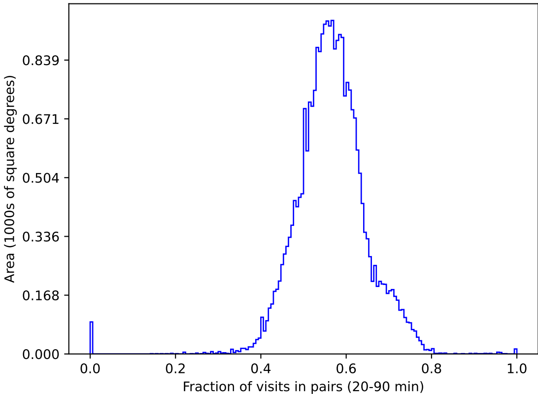
retro_baseline_v2.0_10yrs gri All sky: Fraction of visits in pairs (20-90 min)
