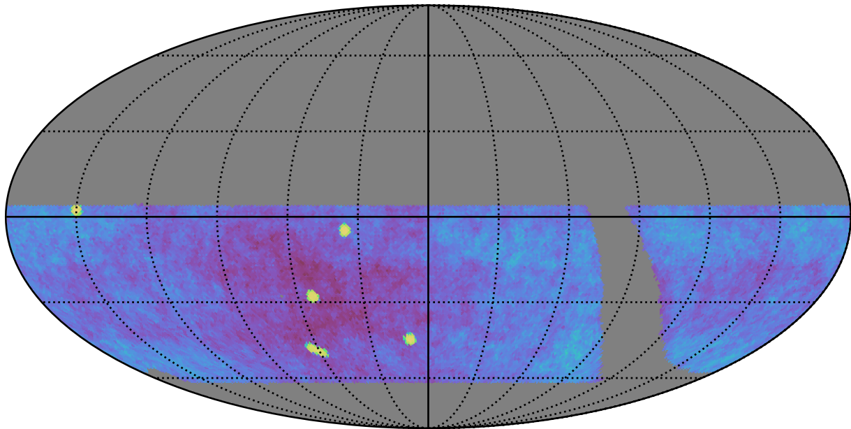
retro_baseline_v2.0_10yrs gri WFD: Fraction of visits in pairs (10-60 min)
