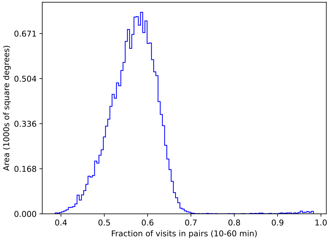
retro_baseline_v2.0_10yrs gri WFD: Fraction of visits in pairs (10-60 min)
