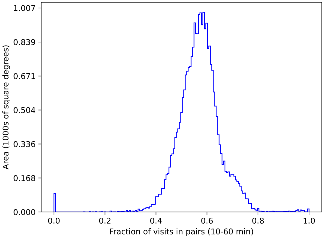
retro_baseline_v2.0_10yrs gri All sky: Fraction of visits in pairs (10-60 min)
