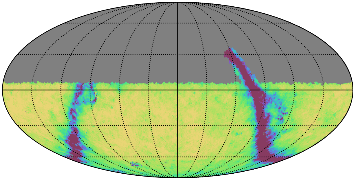
retro_baseline_v2.0_10yrs Yr 3-4 u band: Exgal_CoaddM5
