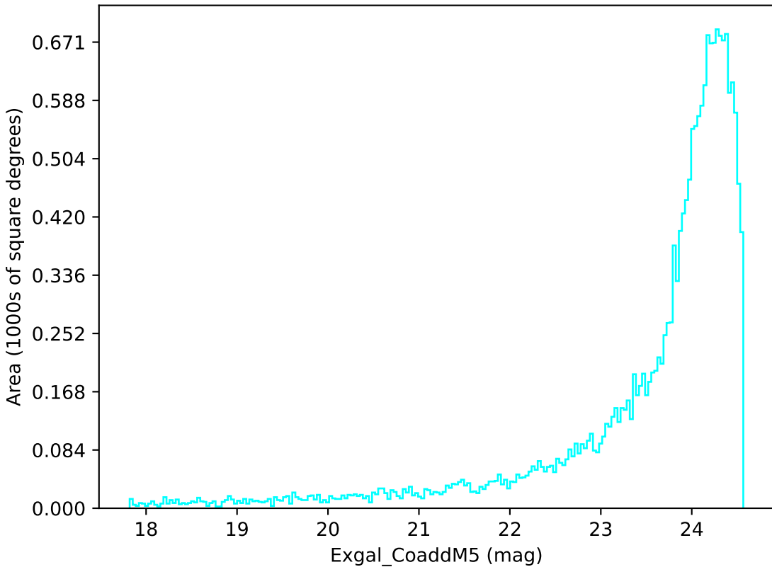
retro_baseline_v2.0_10yrs Yr 3-4 u band: Exgal_CoaddM5
