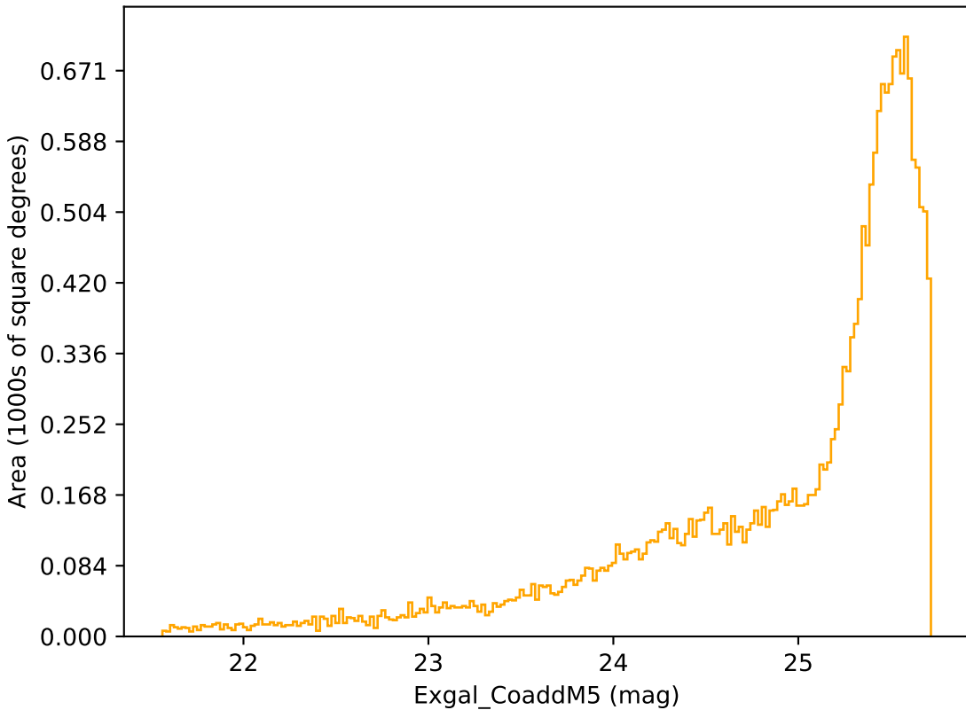
retro_baseline_v2.0_10yrs Yr 3-4 r band: Exgal_CoaddM5
