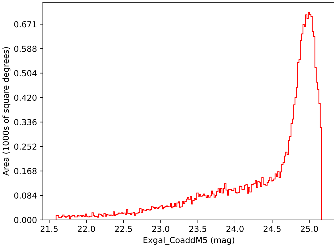
retro_baseline_v2.0_10yrs Yr 3-4 i band: Exgal_CoaddM5
