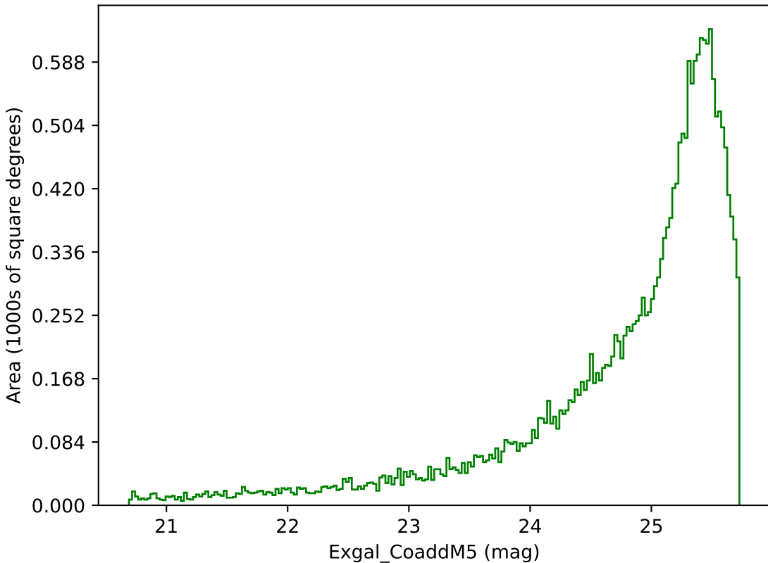
retro_baseline_v2.0_10yrs Yr 3-4 g band: Exgal_CoaddM5
