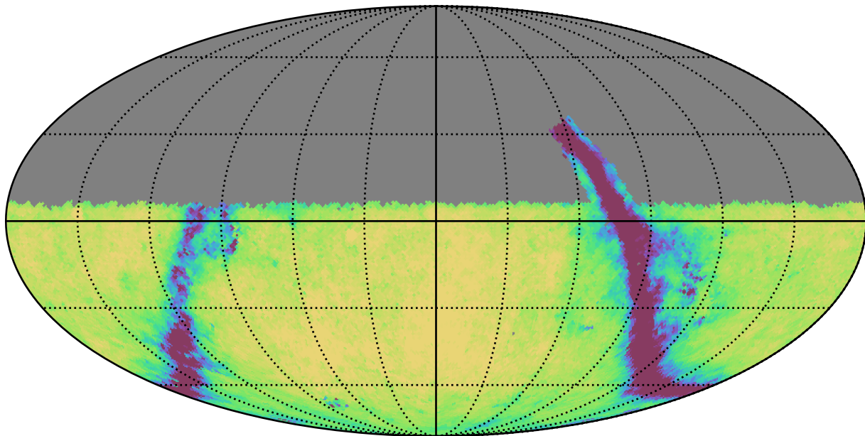
retro_baseline_v2.0_10yrs Yr 1 u band: Exgal_CoaddM5
