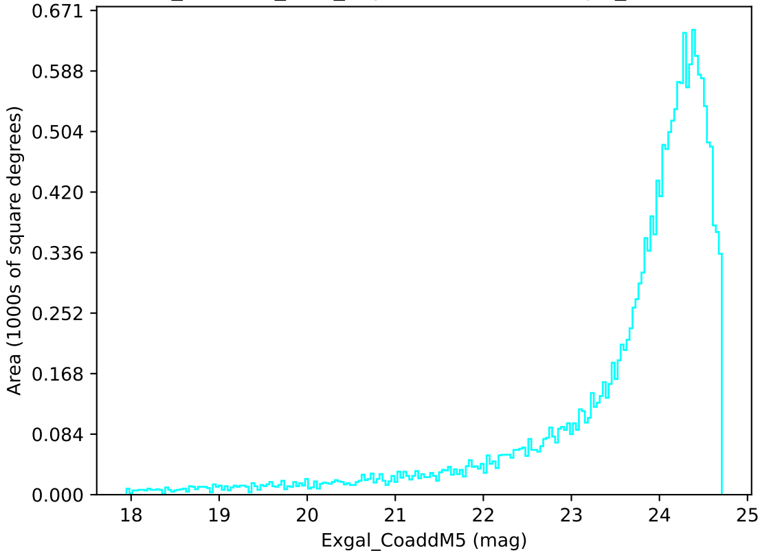
retro_baseline_v2.0_10yrs Yr 1 u band: Exgal_CoaddM5
