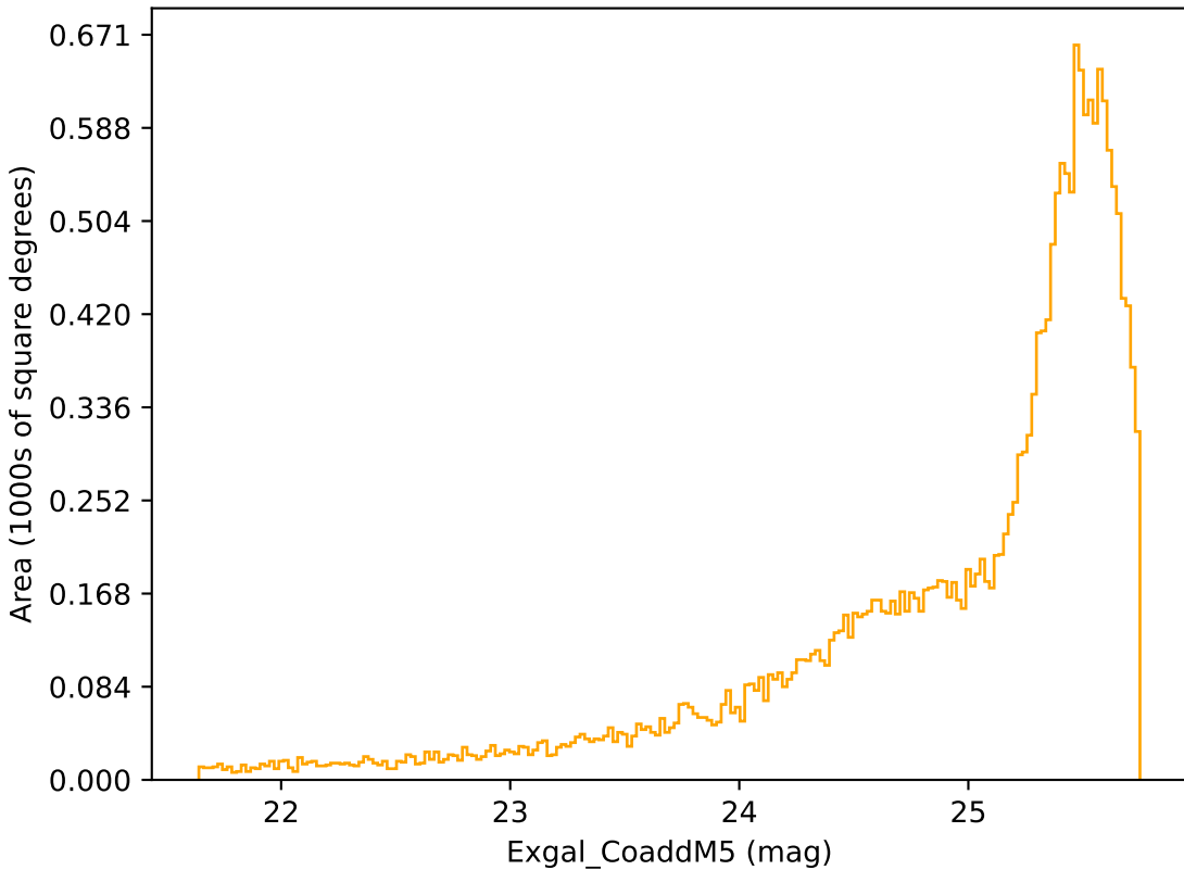
retro_baseline_v2.0_10yrs Yr 1 r band: Exgal_CoaddM5
