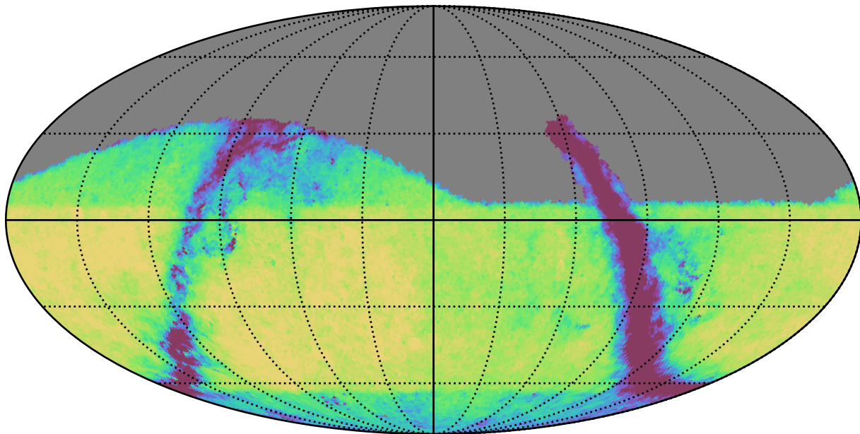
retro_baseline_v2.0_10yrs Yr 1 i band: Exgal_CoaddM5
