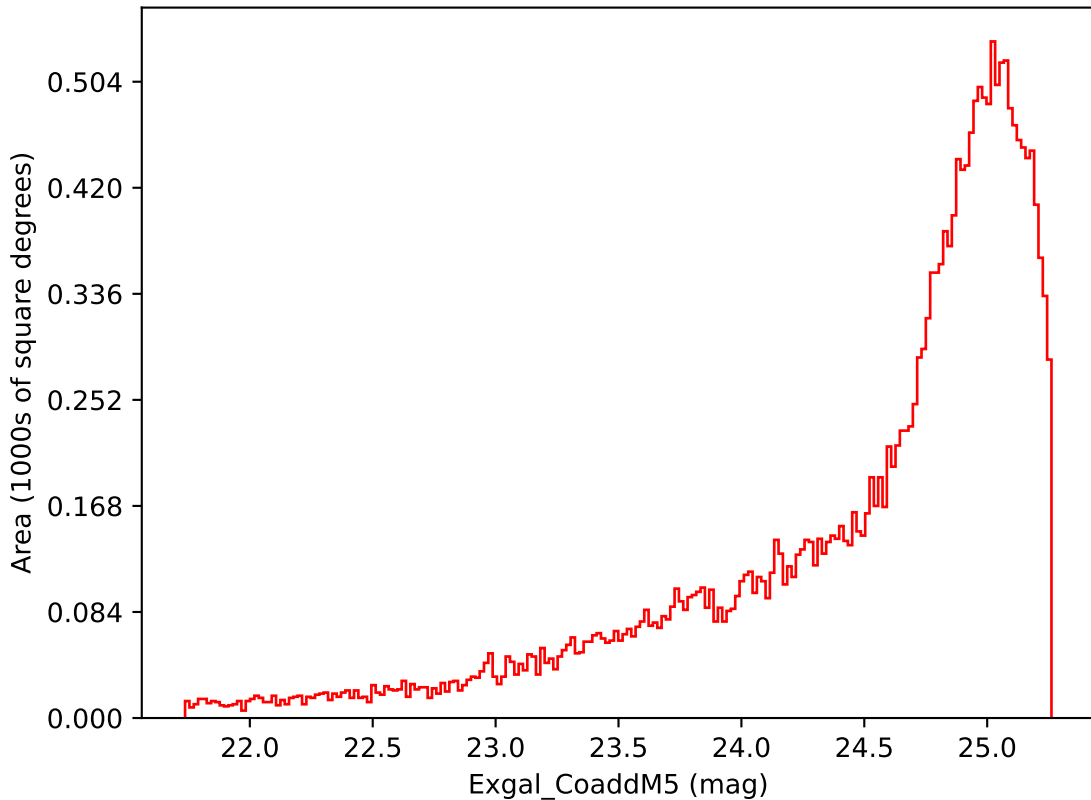
retro_baseline_v2.0_10yrs Yr 1 i band: Exgal_CoaddM5
