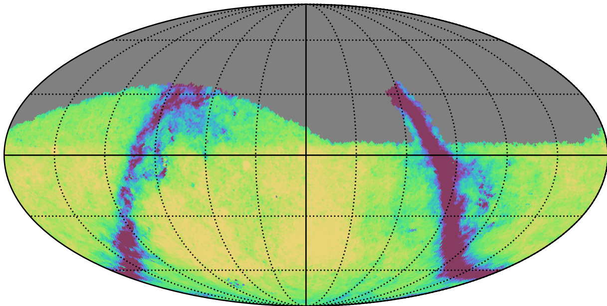
retro_baseline_v2.0_10yrs Yr 1 g band: Exgal_CoaddM5
