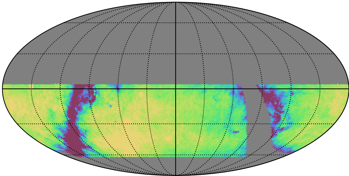
retro_baseline_v2.0_10yrs WFD z band: Exgal_CoaddM5
