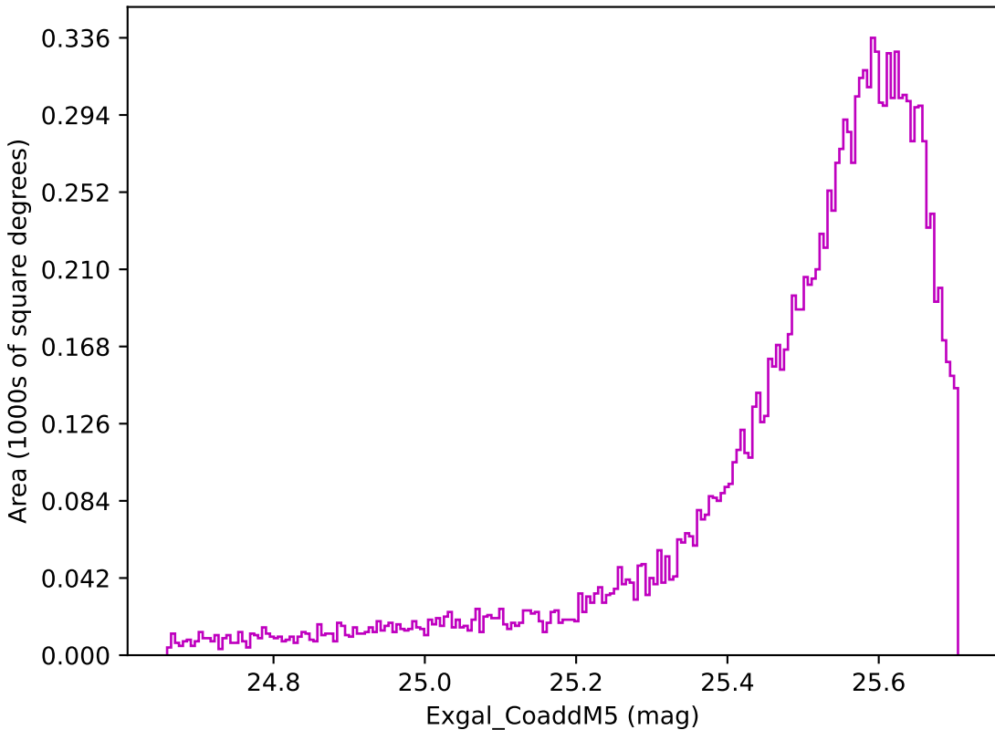
retro_baseline_v2.0_10yrs WFD z band: Exgal_CoaddM5
