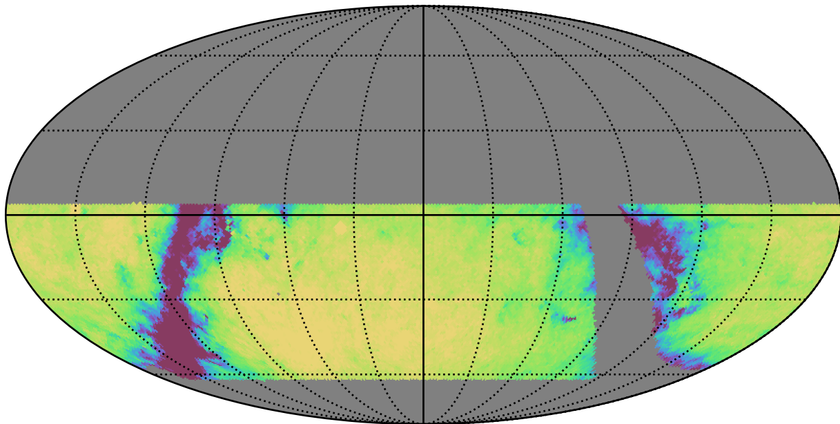
retro_baseline_v2.0_10yrs WFD u band: Exgal_CoaddM5
