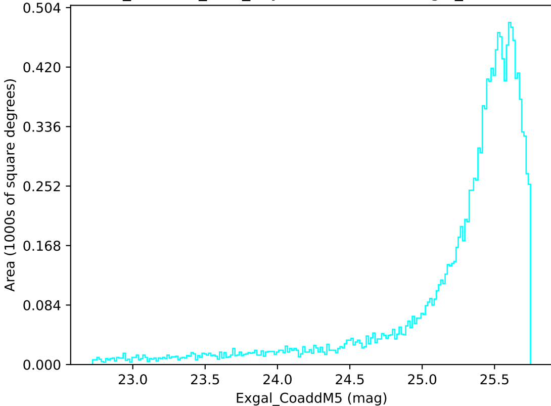
retro_baseline_v2.0_10yrs WFD u band: Exgal_CoaddM5
