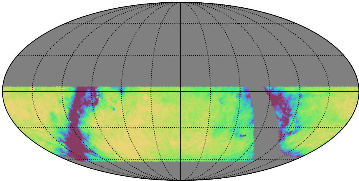
retro_baseline_v2.0_10yrs WFD i band: Exgal_CoaddM5
