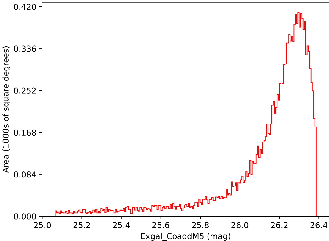
retro_baseline_v2.0_10yrs WFD i band: Exgal_CoaddM5
