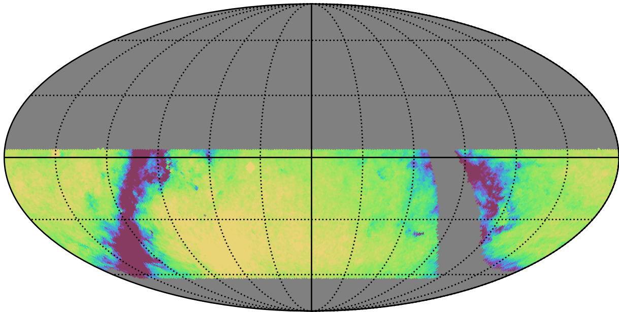
retro_baseline_v2.0_10yrs WFD g band: Exgal_CoaddM5
