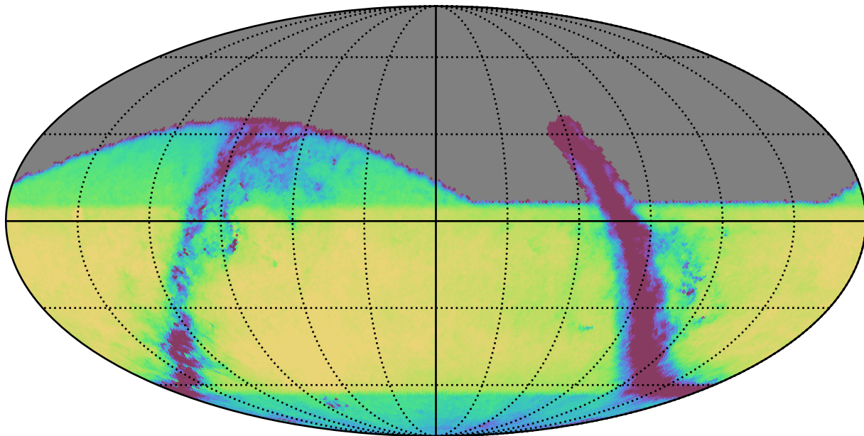
retro_baseline_v2.0_10yrs All sky z band: Exgal_CoaddM5
