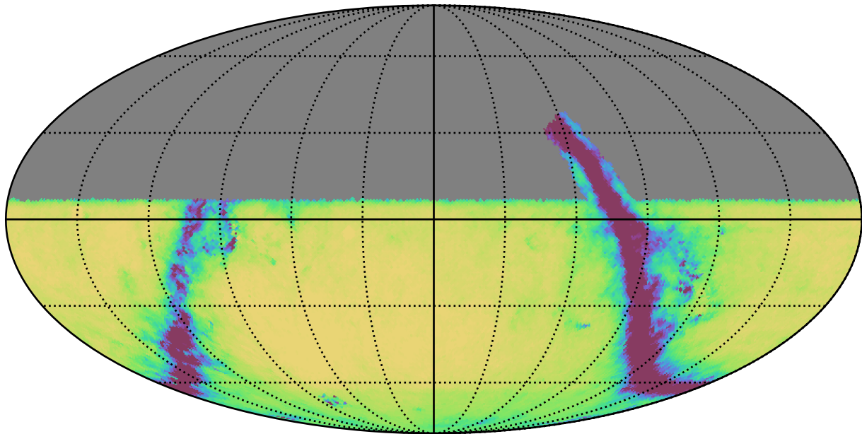
retro_baseline_v2.0_10yrs All sky u band: Exgal_CoaddM5
