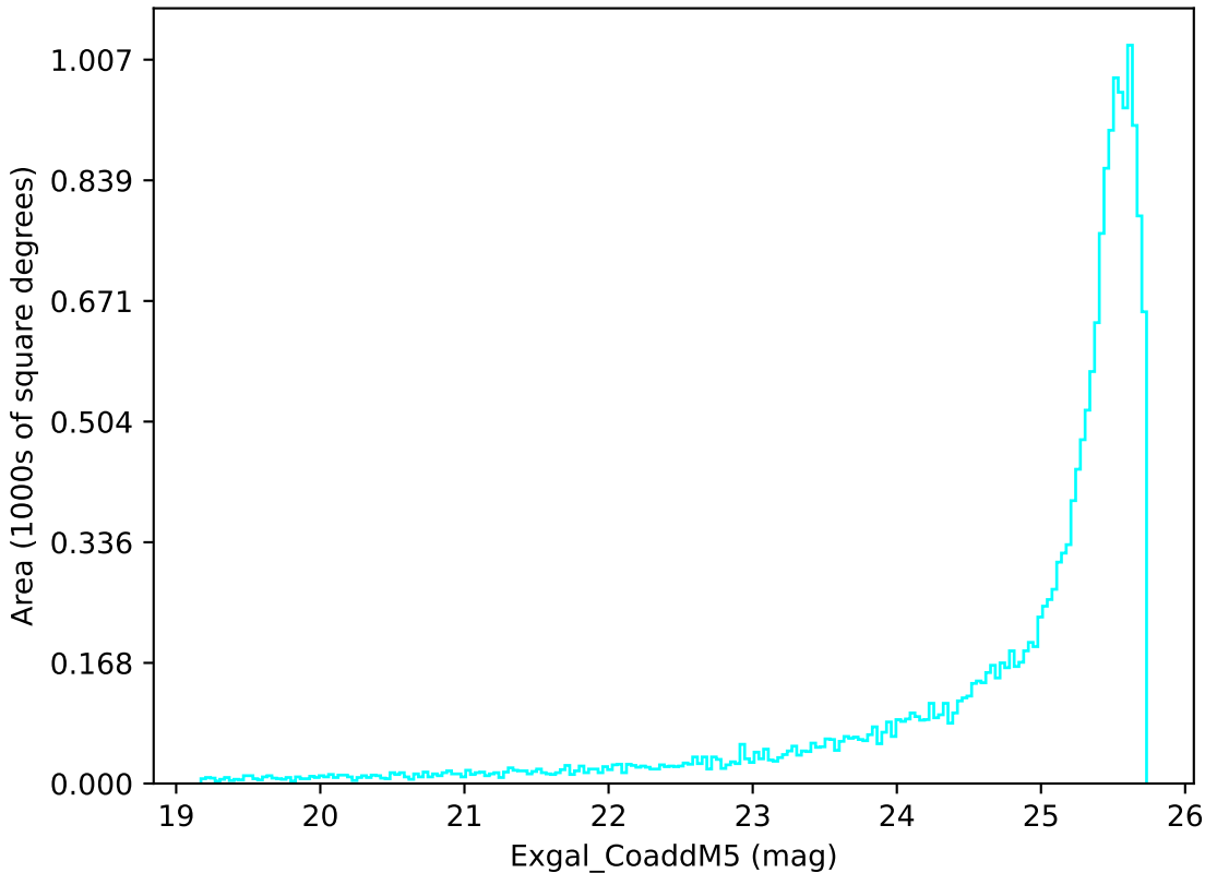
retro_baseline_v2.0_10yrs All sky u band: Exgal_CoaddM5
