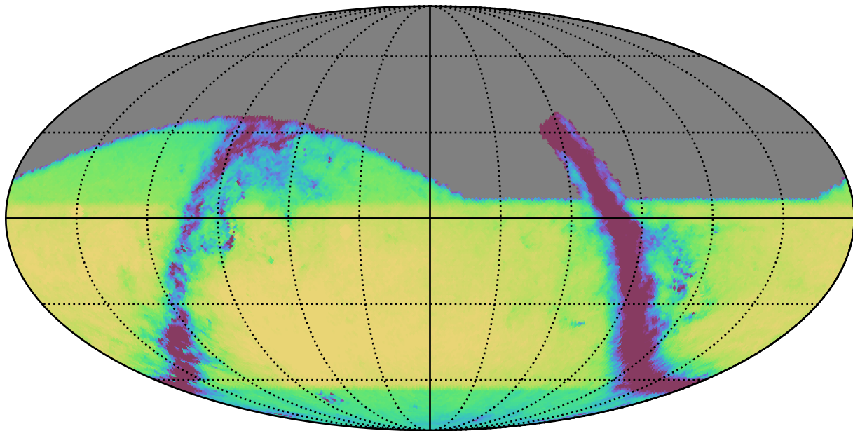
retro_baseline_v2.0_10yrs All sky r band: Exgal_CoaddM5
