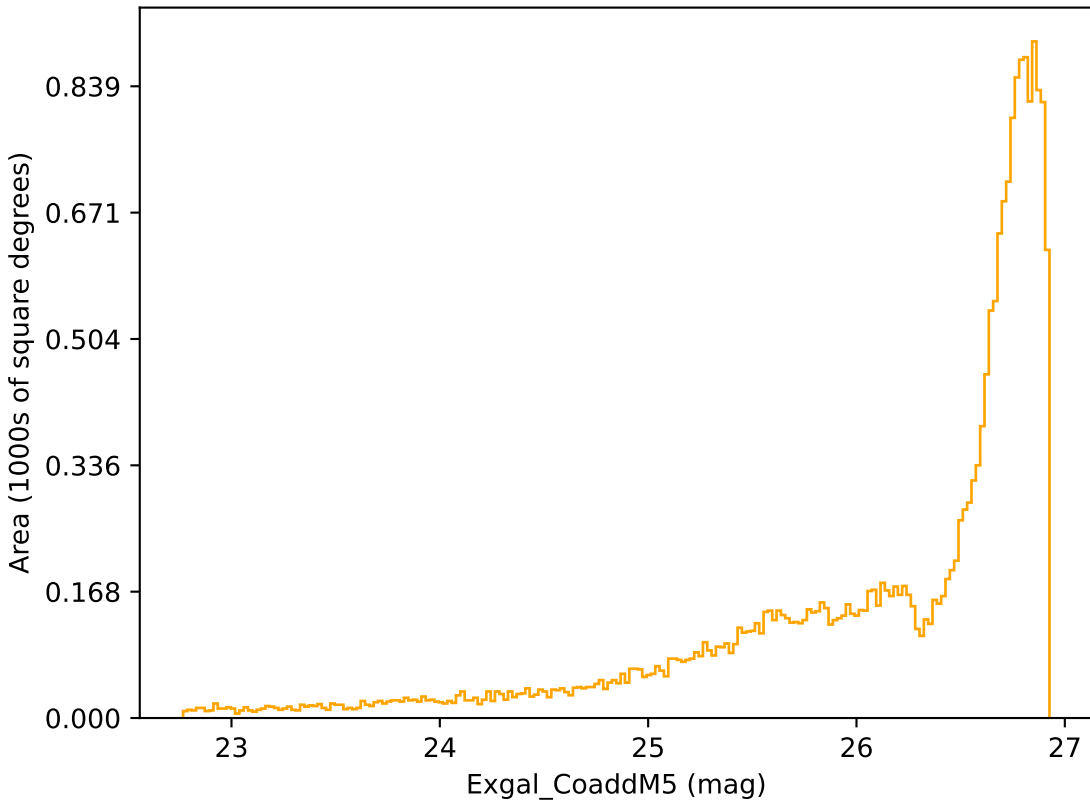
retro_baseline_v2.0_10yrs All sky r band: Exgal_CoaddM5
