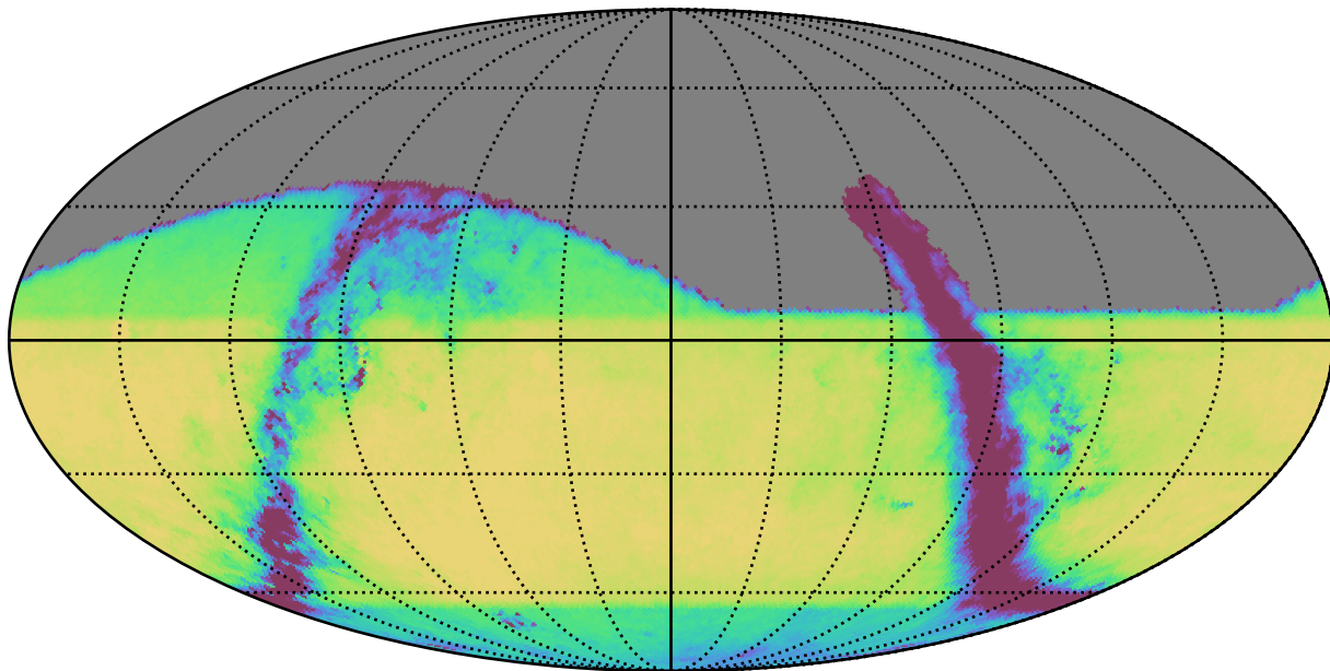
retro_baseline_v2.0_10yrs All sky i band: Exgal_CoaddM5
