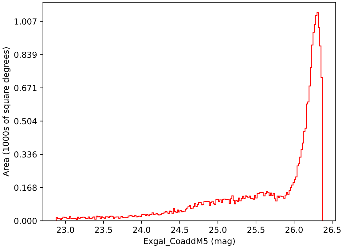
retro_baseline_v2.0_10yrs All sky i band: Exgal_CoaddM5
