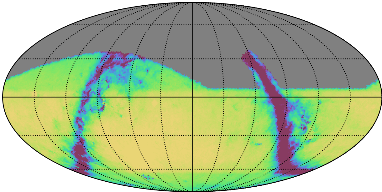
retro_baseline_v2.0_10yrs All sky g band: Exgal_CoaddM5
