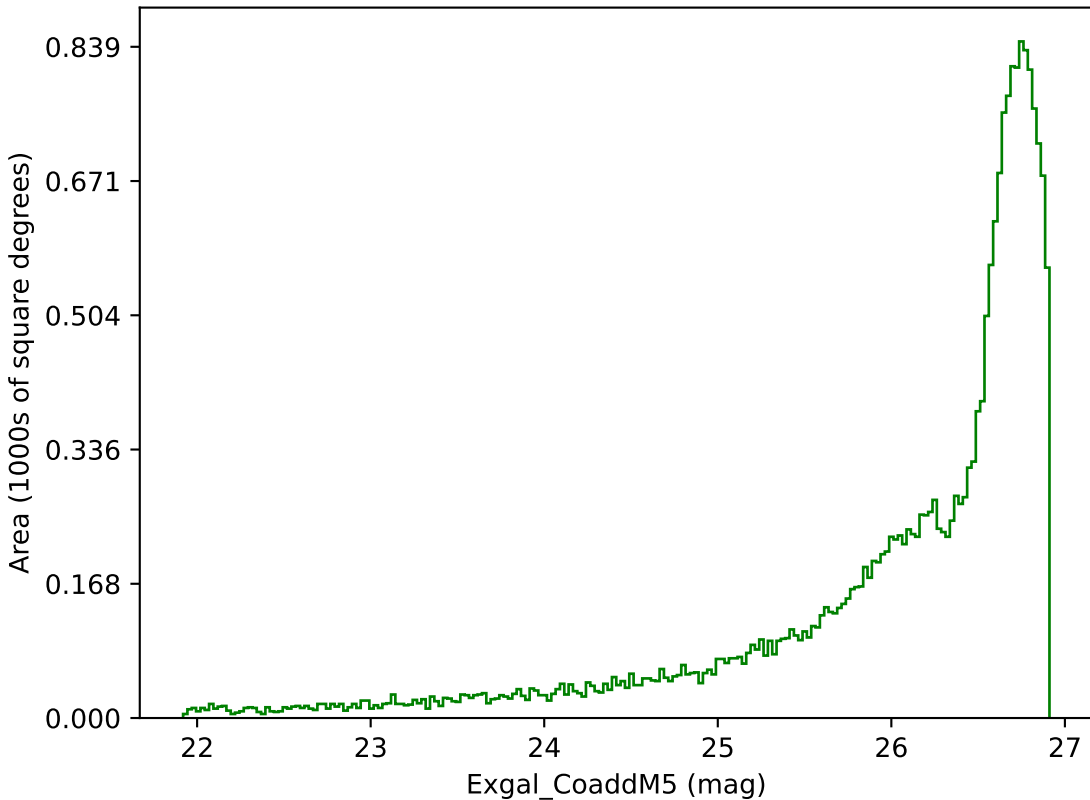
retro_baseline_v2.0_10yrs All sky g band: Exgal_CoaddM5
