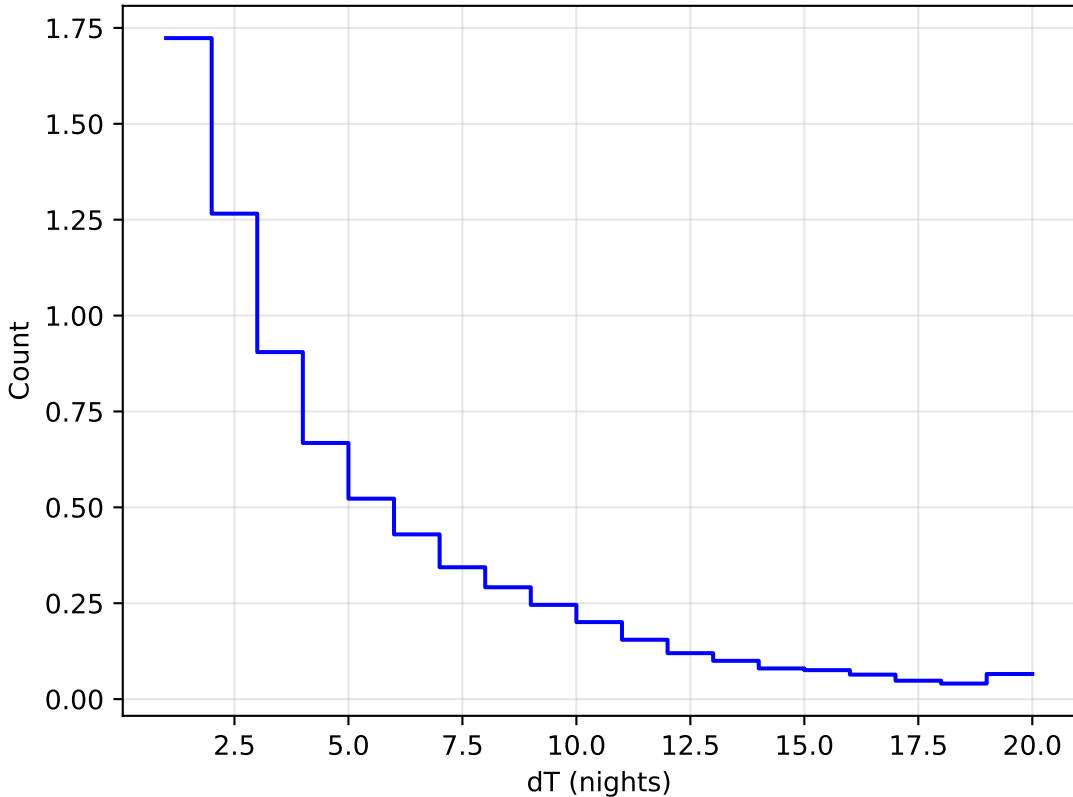
retro_baseline_v2.0_10yrs WFD all bands: DeltaNight Histogram
