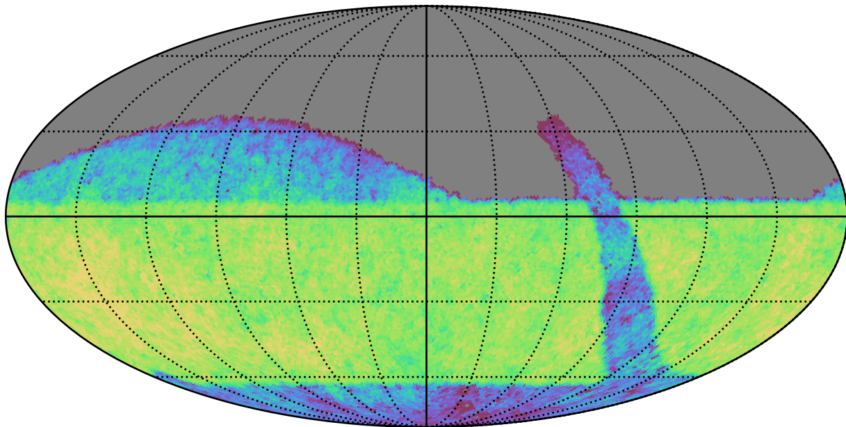
retro_baseline_v2.0_10yrs Yr 3-4 z band: CoaddM5
