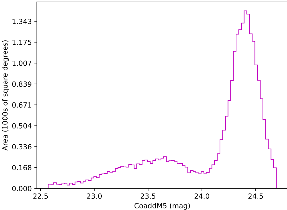
retro_baseline_v2.0_10yrs Yr 3-4 z band: CoaddM5
