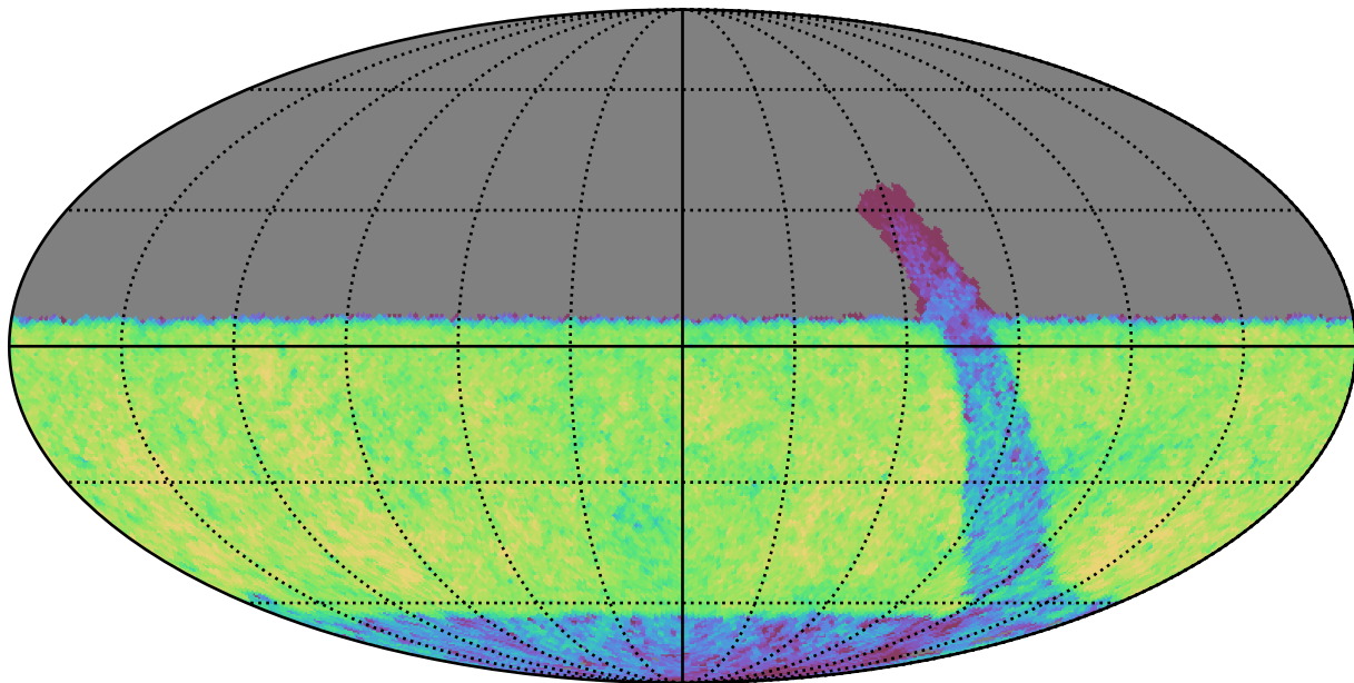
retro_baseline_v2.0_10yrs Yr 3-4 y band: CoaddM5
