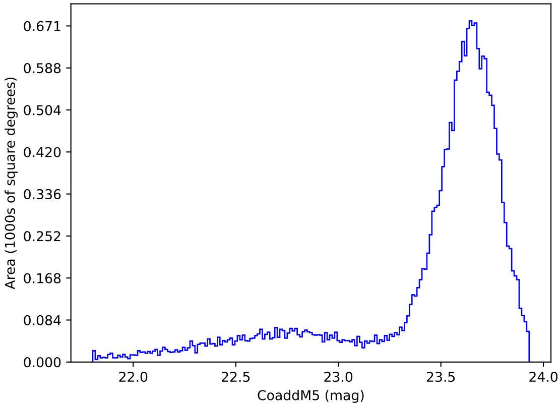
retro_baseline_v2.0_10yrs Yr 3-4 y band: CoaddM5
