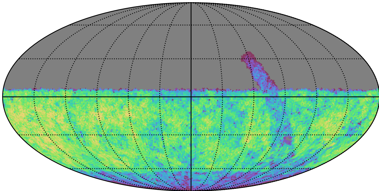
retro_baseline_v2.0_10yrs Yr 3-4 u band: CoaddM5
