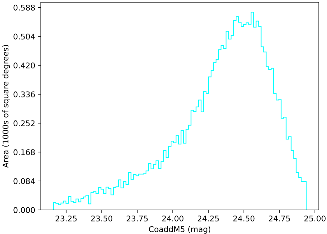
retro_baseline_v2.0_10yrs Yr 3-4 u band: CoaddM5
