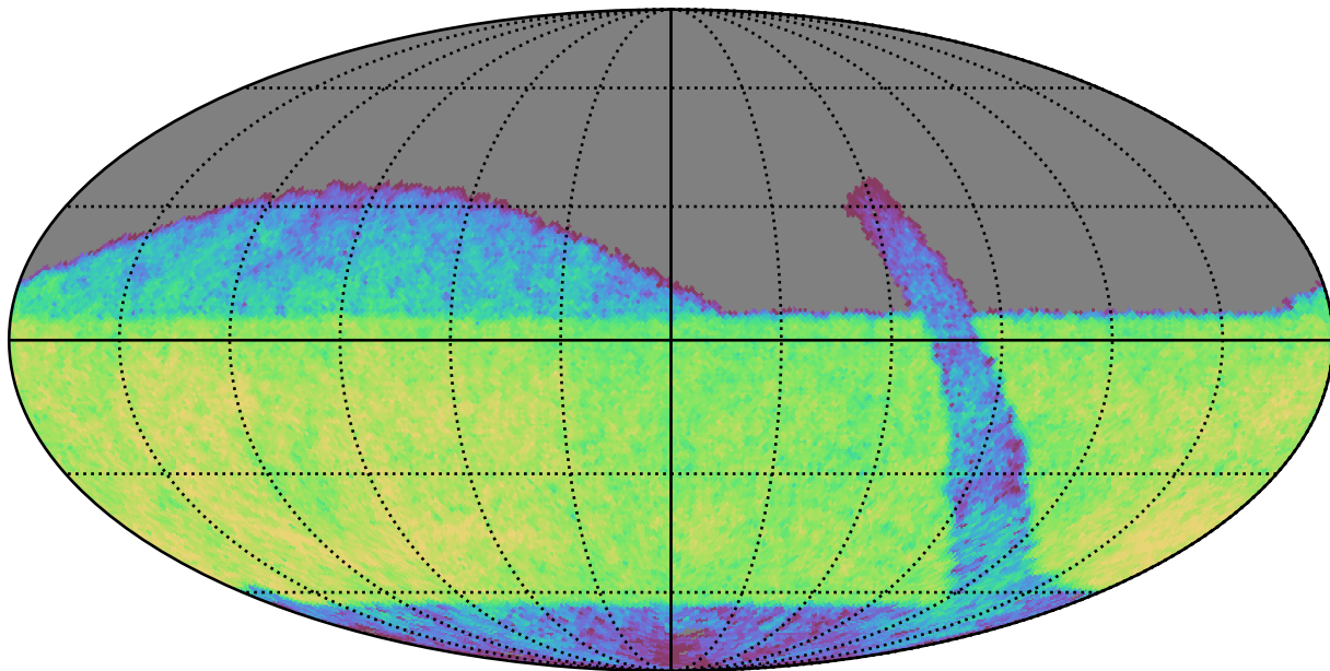
retro_baseline_v2.0_10yrs Yr 3-4 r band: CoaddM5
