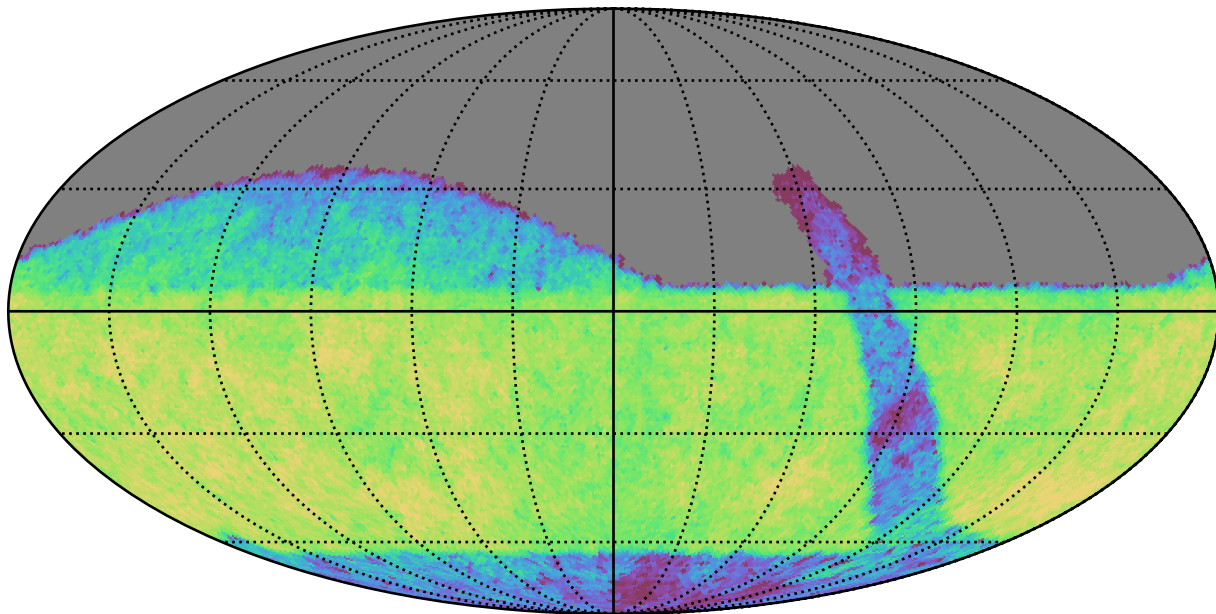
retro_baseline_v2.0_10yrs Yr 3-4 i band: CoaddM5
