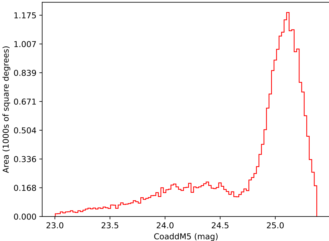
retro_baseline_v2.0_10yrs Yr 3-4 i band: CoaddM5
