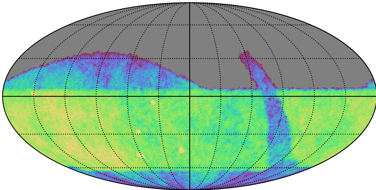
retro_baseline_v2.0_10yrs Yr 1 z band: CoaddM5
