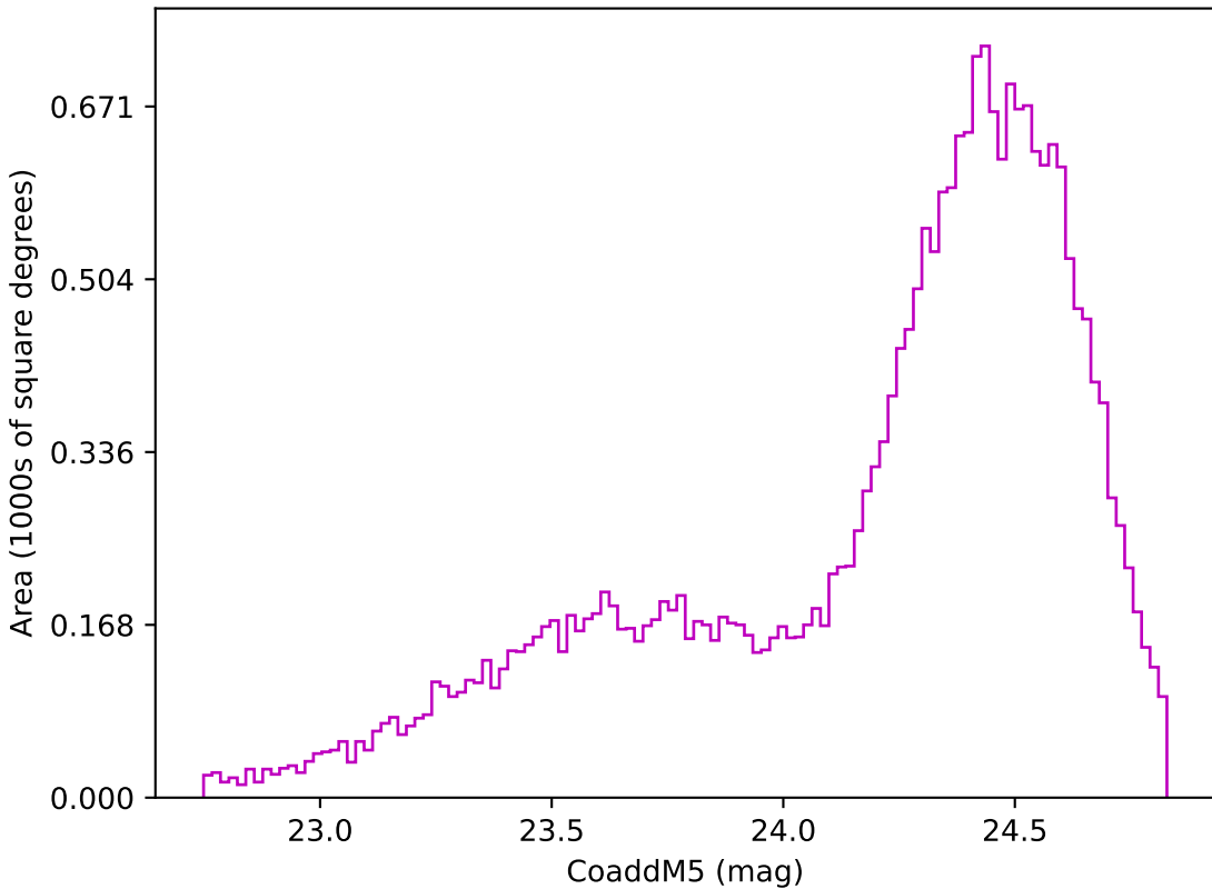
retro_baseline_v2.0_10yrs Yr 1 z band: CoaddM5
