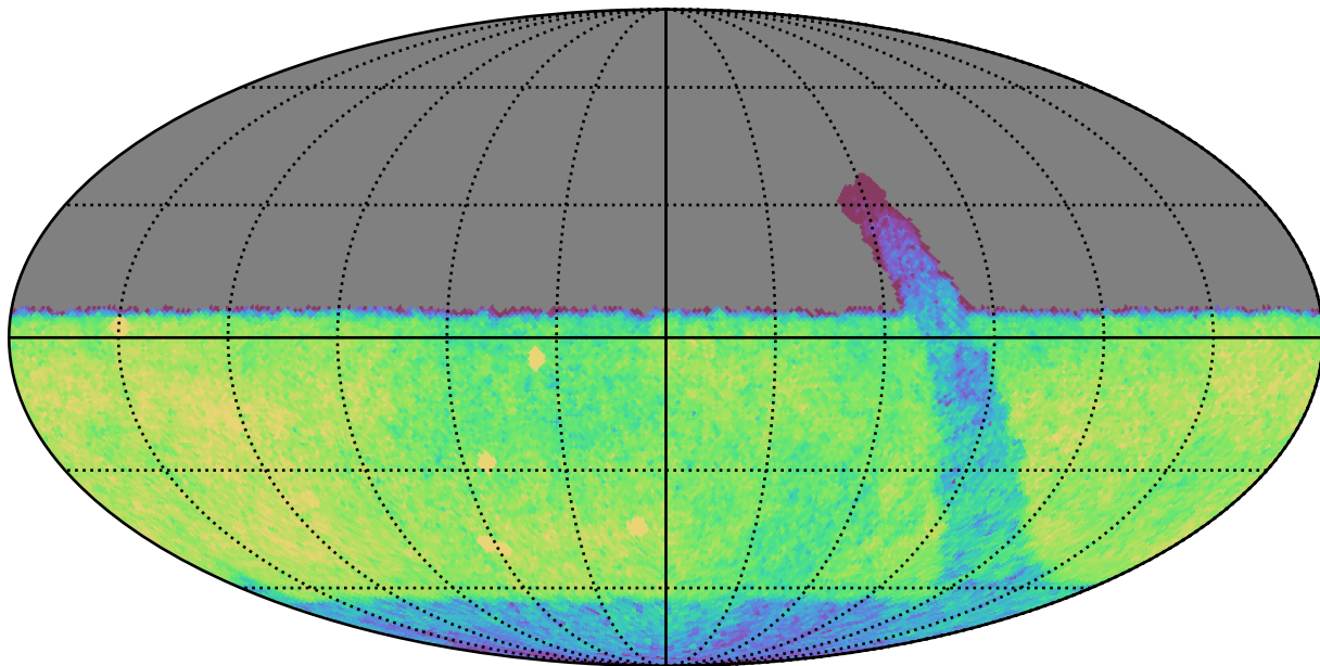
retro_baseline_v2.0_10yrs Yr 1 y band: CoaddM5
