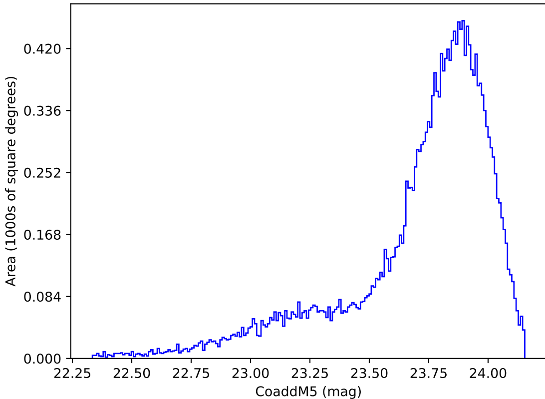
retro_baseline_v2.0_10yrs Yr 1 y band: CoaddM5
