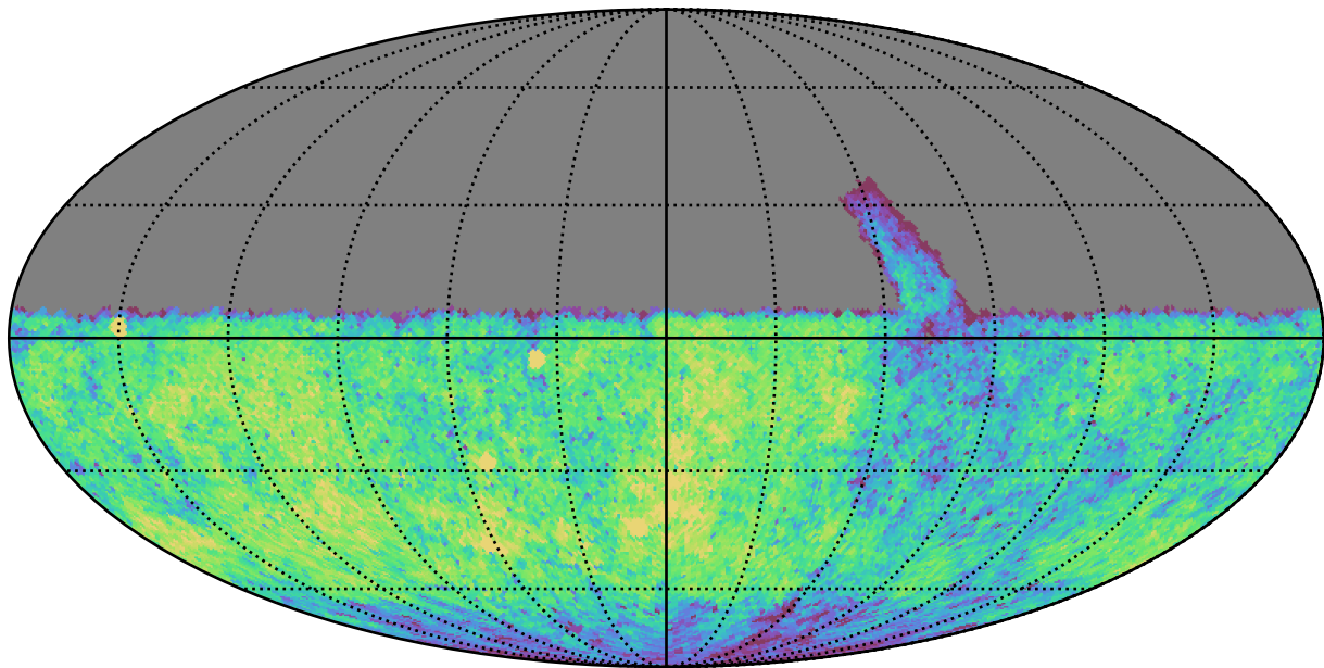
retro_baseline_v2.0_10yrs Yr 1 u band: CoaddM5
