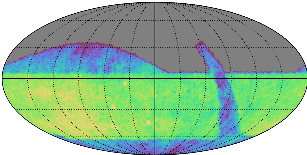
retro_baseline_v2.0_10yrs Yr 1 r band: CoaddM5
