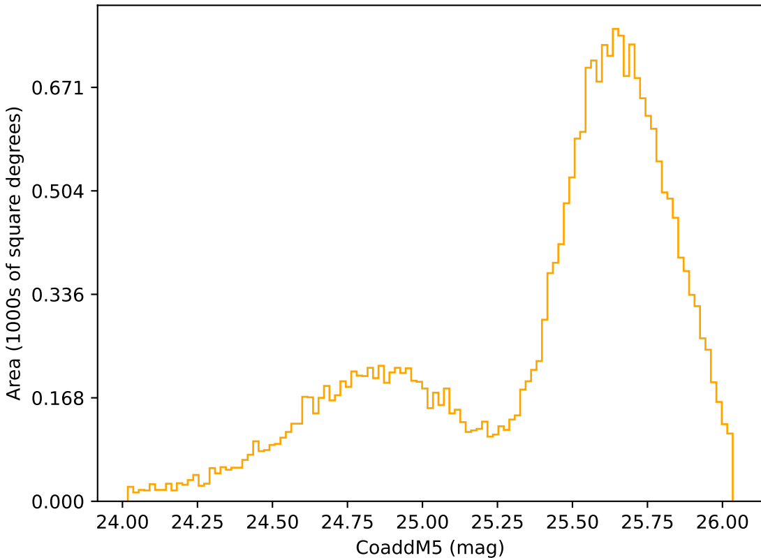
retro_baseline_v2.0_10yrs Yr 1 r band: CoaddM5
