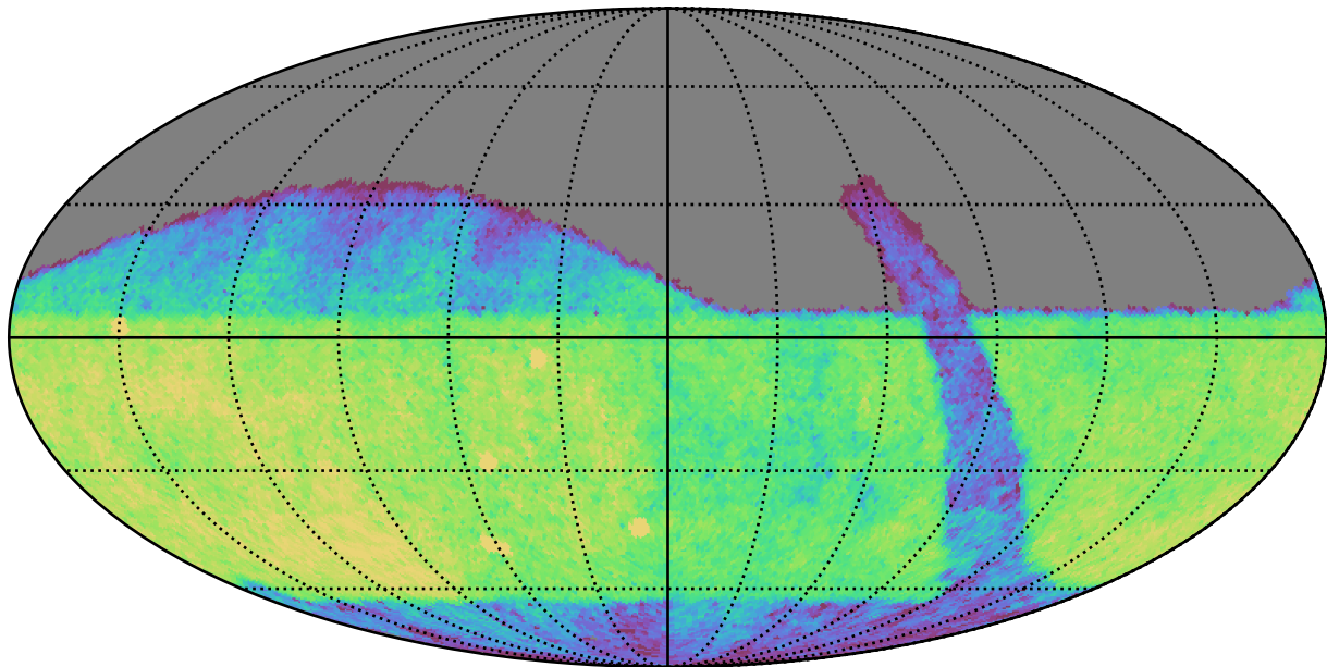
retro_baseline_v2.0_10yrs Yr 1 i band: CoaddM5
